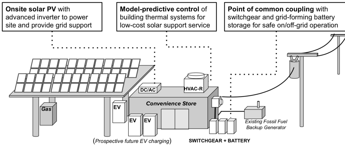
Figure 2: Conceptual diagram of pilot Solar+ microgrid including notes on key features. Existing site components are shaded and new components are white.
